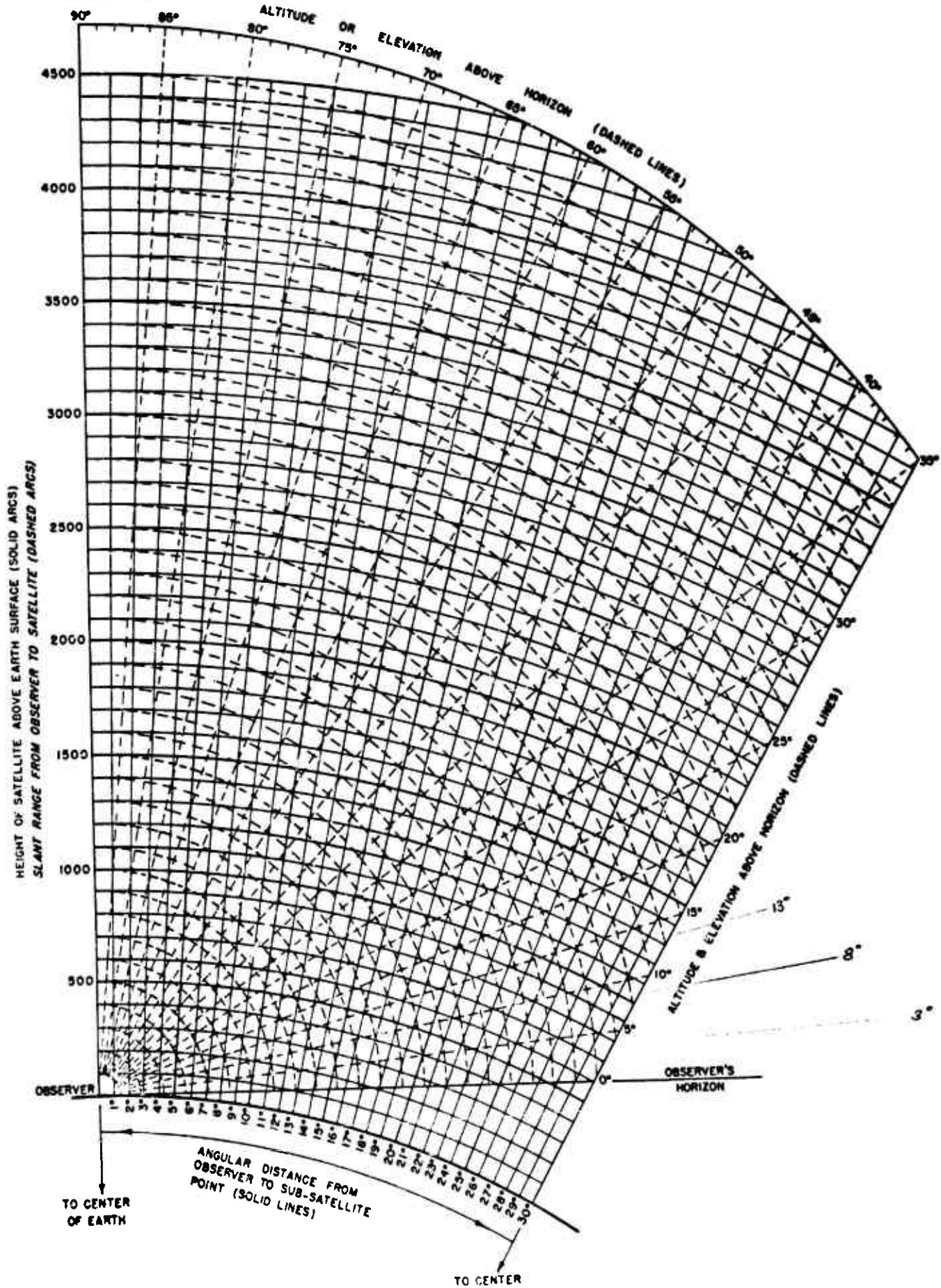
CHART FOR DETERMINING ELEVATION & SLANT RANGE OF SATELLITE
