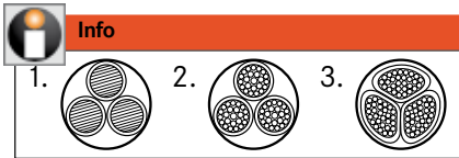
1. re = round conductor, single wire; 2. rm = round conductor, multi wire; 3. sm = sectorial conductor
