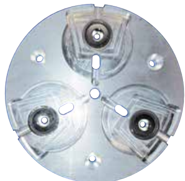
UNIVERSAL MAGNETIC PLATE FOR SKANMASKIN® 8.25" Universal Magnetic Plate AUPSK-650-8
