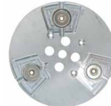
UNIVERSAL MAGNETIC PLATE FOR LAVINA® 21-1.5, 21-3 8" Universal Magnetic Plate AUPL-8
