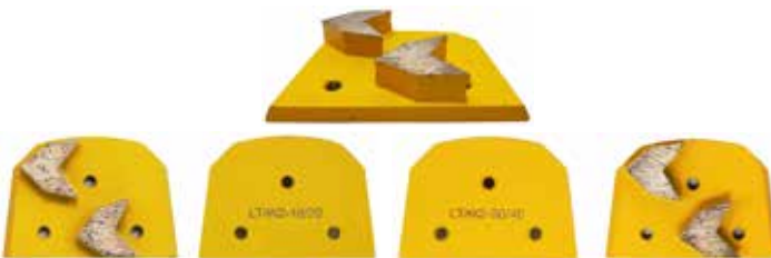
LAVINA® STYLE DOUBLE ARROW 2X-EXTREME SOFT BOND (YELLOW)
