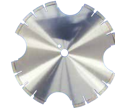
14" NINJA cleanout blade x .250" NB14-10
