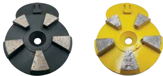
3" STI® STYLE - 5 BEVELED SEGMENTS MEDIUM BOND (BLACK)
