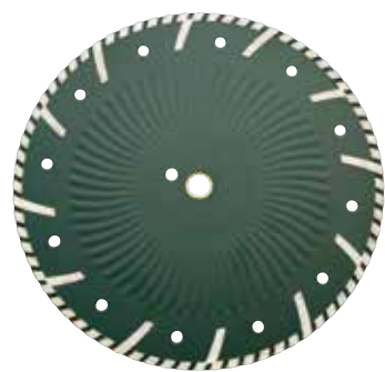
SUPER TURBO General Purpose, Dry/Wet 12" x .125" x 1" / 20mm STGP12-H 14" x .125" x 1" / 20mm STGP14-H
