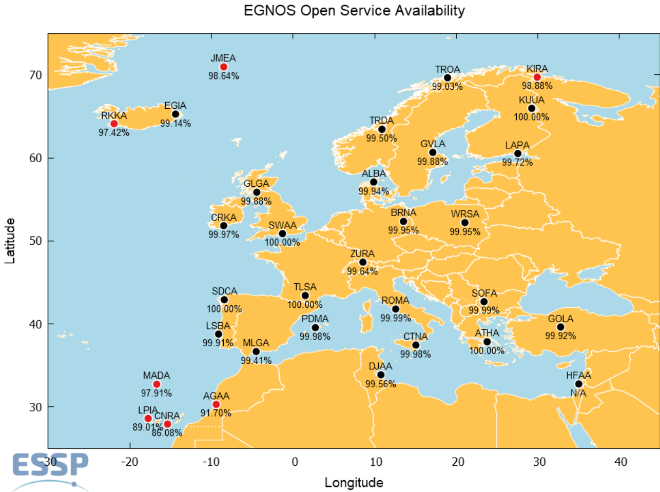
Figure 5 – EGNOS Open Service Availability at reference stations 3
