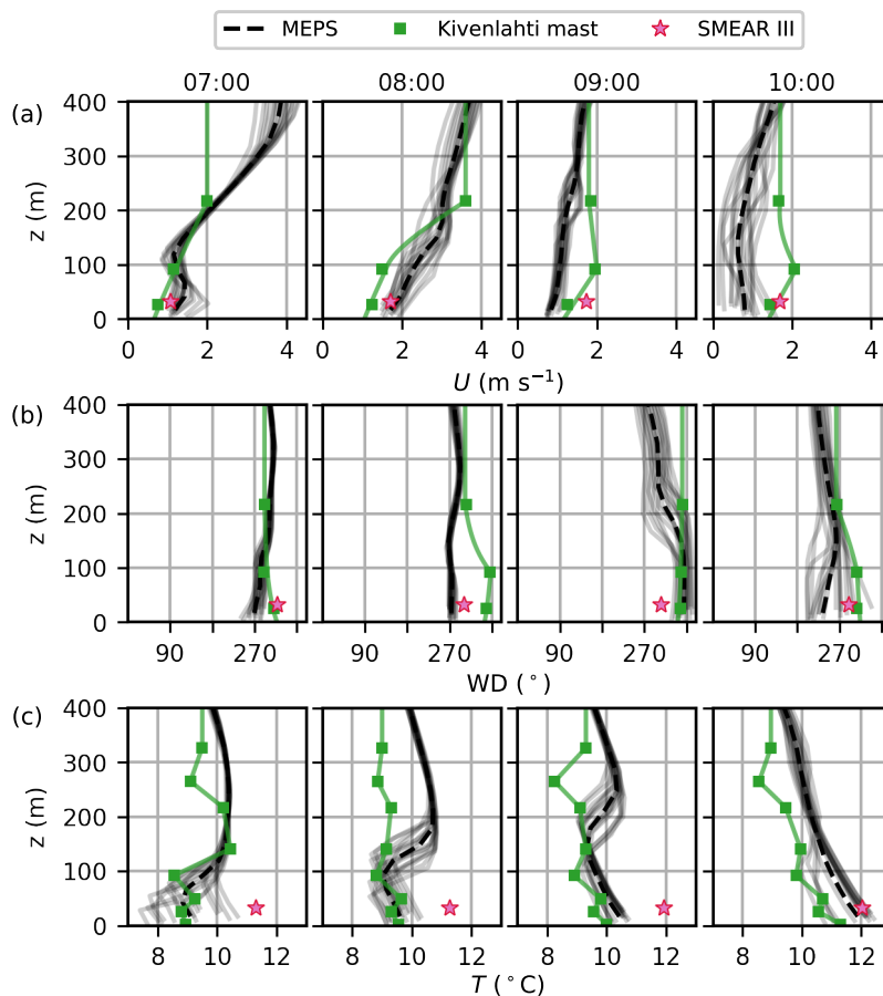
Figure 2. Horizontal a) wind speed U ( \text{m s}^{-1} ), b) wind direction WD ( ^{\circ} ) and c) air temperature T ( ^{\circ}\text{C} ) on 9 Jun at local time (UTC+3). The modelled profiles at each MEPS grid point are shown by grey solid lines and their mean by a black dashed line. The observation from the Kivenlahti mast are shown by green solid squares and the interpolated profiles used as boundary conditions by a green solid line. Stars show the SMEAR III observations.
