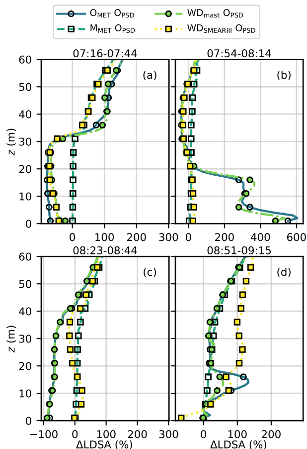
Figure 11. Relative difference in the lung-deposited surface area ( \Delta\text{LDSA} ) of aerosol particles compared to M_{\text{MET}}M_{\text{PSD}} at the supersite (a,c) and opposite supersite (b,d) on 9 Jun morning. The figure shows the difference in the geometric mean for O_{\text{MET}}O_{\text{PSD}} (solid line with empty circles), M_{\text{MET}}O_{\text{PSD}} (dashed line with empty squares), O_{\text{WD,mast}}O_{\text{PSD}} (dash-dot line with filled squares) and O_{\text{WD,SMEAR}}O_{\text{PSD}} (dotted line with filled squares).
