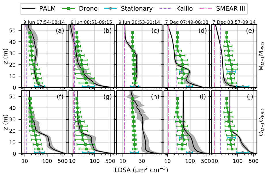
Figure 6. Measured (marker with error bar) and modelled (black line and grey shaded area) lung-deposited surface area (LDSA) of aerosol particles opposite the supersite for the summer morning (a,f for the first and b,g for the second hour), summer evening (c,h) and winter morning (d,i for the first and e,j for the second hour). The first row shows M_{MET}M_{PSD} and the second O_{MET}O_{PSD} . The figure shows the geometric mean (measured: marker, modelled: solid line) and geometric standard deviation (measured: error bar, modelled: shaded area). Dashed lines show the geometric mean at the urban background monitoring sites in Kallio and SMEAR III.
