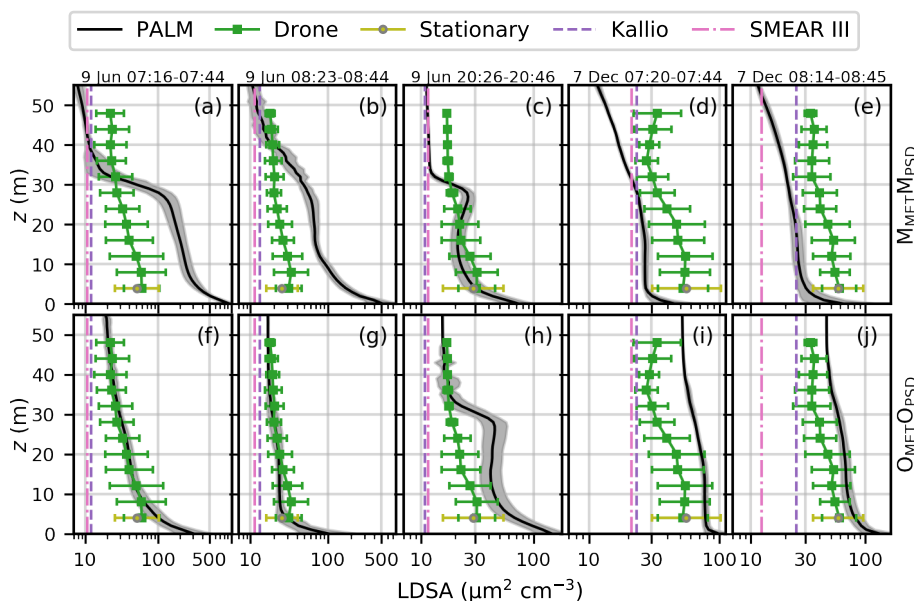
Figure 5. Measured (marker with error bar) and modelled (black line and grey shaded area) lung-deposited surface area (LDSA) of aerosol particles at the supersite for the summer morning (a,f for the first and b,g for the second hour), summer evening (c,h) and winter morning (d,i for the first and e,j for the second hour). The first row shows M_{MET}M_{PSD} and the second O_{MET}O_{PSD} . The figure shows the geometric mean (measured: marker, modelled: solid line) and geometric standard deviation (measured: error bar, modelled: shaded area). Dashed lines show the geometric mean at the urban background monitoring sites in Kallio and SMEAR III.
