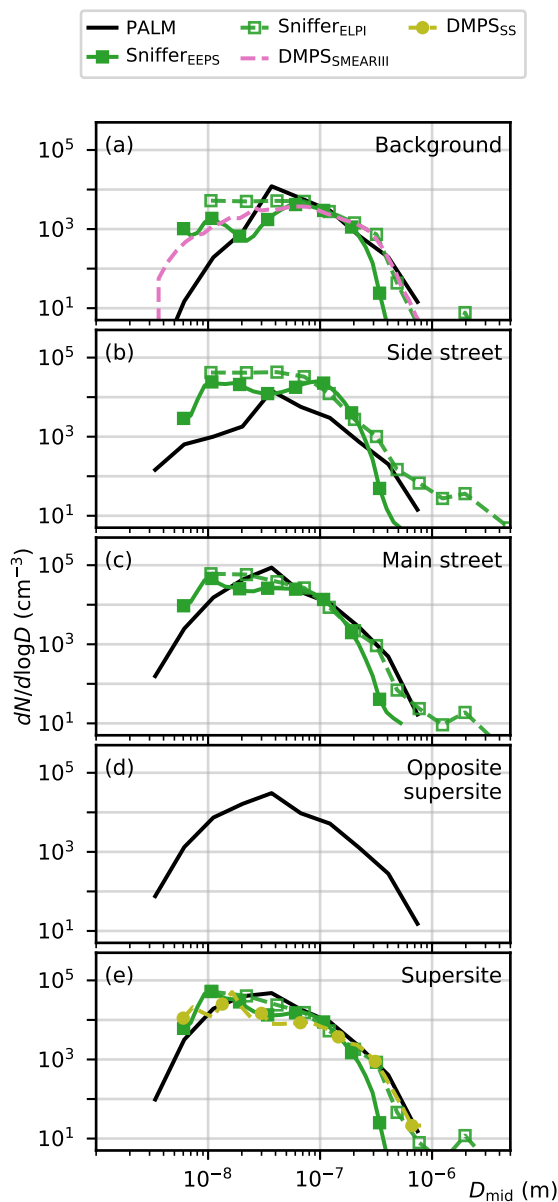
Figure 9. The mean aerosol number size distribution dN/d\log D ( \text{cm}^{-3} ) at different parts of the domain at z = 1.5 m for M_{\text{MET}}M_{\text{PSD}} on 9 Jun morning at 07:16–08:14. Modelled values are shown with a black solid line and Sniffer measurements with green lines: solid with filled squares for EEPS and dotted with empty squares for ELPI. Stationary DMPS measurements are shown with a light-green solid line with circles (SS = supersite) and pink dotted line (SMEAR III). Note that for this observation period no stationary Sniffer measurements are available opposite the supersite.
