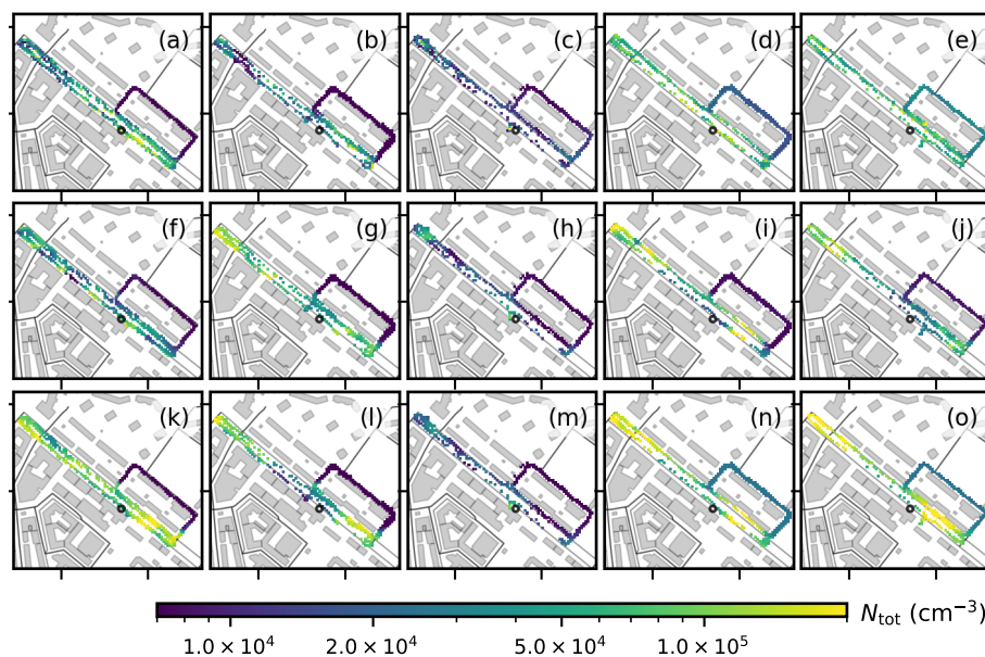
Figure 3. Measured (a-e) and modelled (f-o) total aerosol number concentration ( N_{tot} ) along the Sniffer route for the summer morning (a,f,k for the first and b,g,l for the second hour), summer evening (c,h,m) and winter morning (d,i,n for the first and e,j,o for the second hour). The second row shows M_{MET}M_{PSD} and the third O_{MET}O_{PSD} . Measurements are from z = 2.4 m and modelled values from z = 2.5 m. The supersite is marked with a black circle. Note the different scale in different columns.
