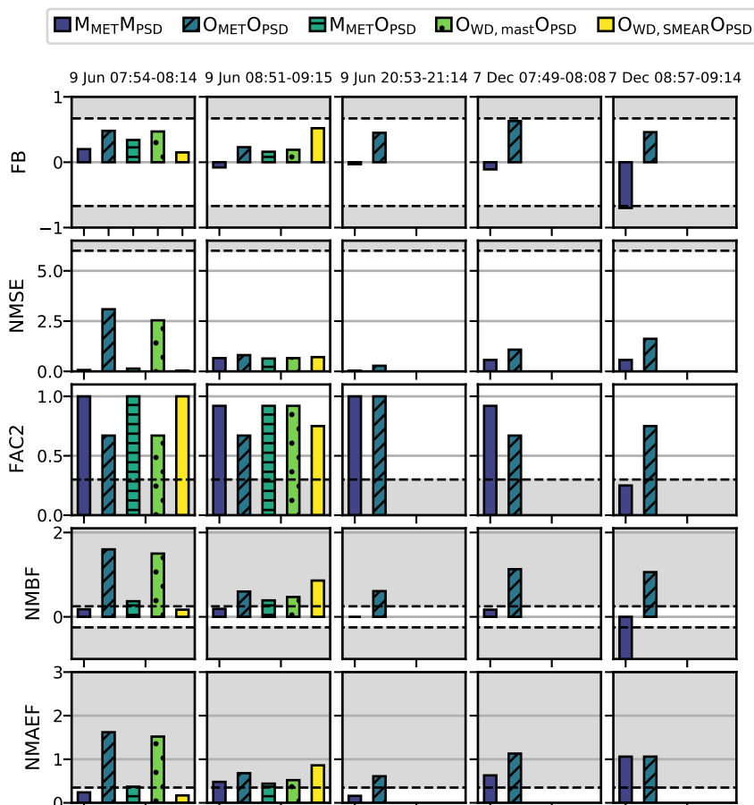
Figure 8. Model performance for the vertical distribution of LDSA opposite the supersite. The grey indicates that the value exceeds the acceptance criteria given in Table 5. See Fig. 4 for details.
