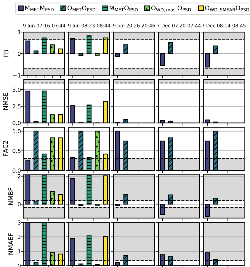
Figure 7. Model performance for the vertical distribution of LDSA at the supersite. The grey indicates that the value exceeds the acceptance criteria given in Table 5. See Fig. 4 for details.
