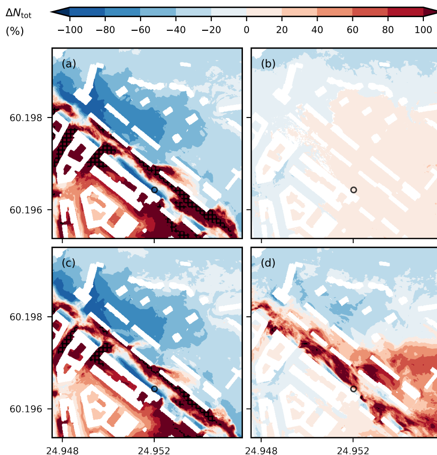
Figure 10. Relative difference in the total aerosol number concentration ( \Delta N_{\text{tot}} ) at z = 2.5 m on 9 Jun morning between 07:16–09:15 am compared to M_{\text{MET}}M_{\text{PSD}} for a) O_{\text{MET}}O_{\text{PSD}} , b) M_{\text{MET}}O_{\text{PSD}} , c) O_{\text{WD,mast}}O_{\text{PSD}} and d) O_{\text{WD,SMEAR}}O_{\text{PSD}} . Area with black crosses show |\Delta N_{\text{tot}}| > 150\% . Buildings are shown with white and black circle denotes the location of the supersite. Note that \Delta N_{\text{tot}} is shown here for the whole simulation and not separately for each hour.
