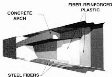
The key components of the hybrid-composite beam
