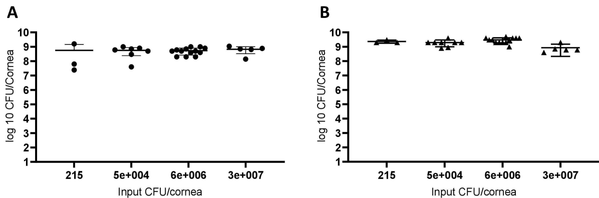
285 286 Fig 2. Number of viable P. aeruginosa PA14 retrieved from porcine cornea after infection with 287 215, 5 \times 10^4 , 6 \times 10^6 and 3 \times 10^7 CFU per cornea. Corneas were infected for 24 hours (A) and 48 288 hours (B). Each dot represents results from one cornea. Error bars represent standard deviation. 289 Statistical significance was calculated with Kruskal-Wallis test followed by Dunn's multiple 290 comparisons test * p -value < 0.05 . Raw data is available in Supplementary Materials, Data 291 Availability Section.
