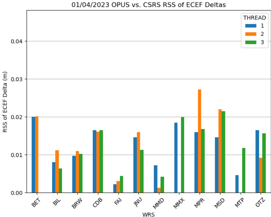
Figure 10-7 OPUS vs. CSRS RSS ECEF Deltas (1 of 3)
