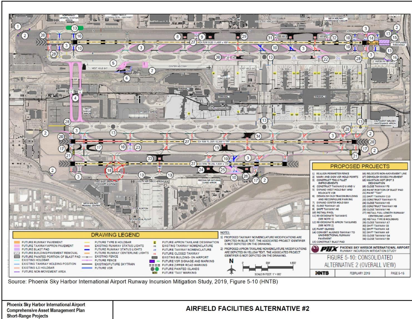
Exhibit 2-3: Airfield Alternative #2
