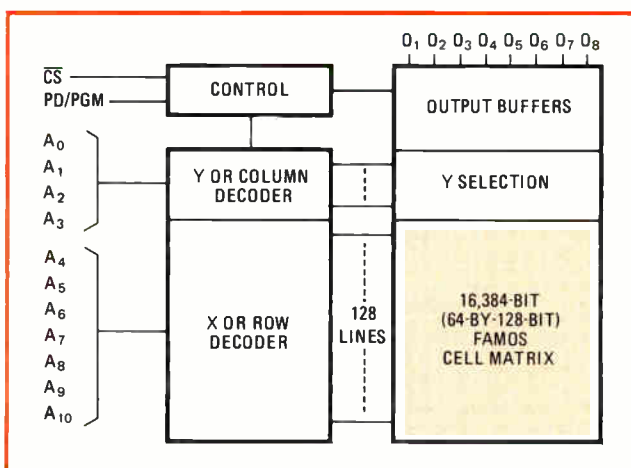
2. Aimed at microcomputers. The 16,384 cells in the 2716 device are organized into two 64-by-128-cell arrays or 2,048 8-bit words, an arrangement that makes the device useful for byte-oriented microcomputer designs and also compatible with 16-k ROMs.
