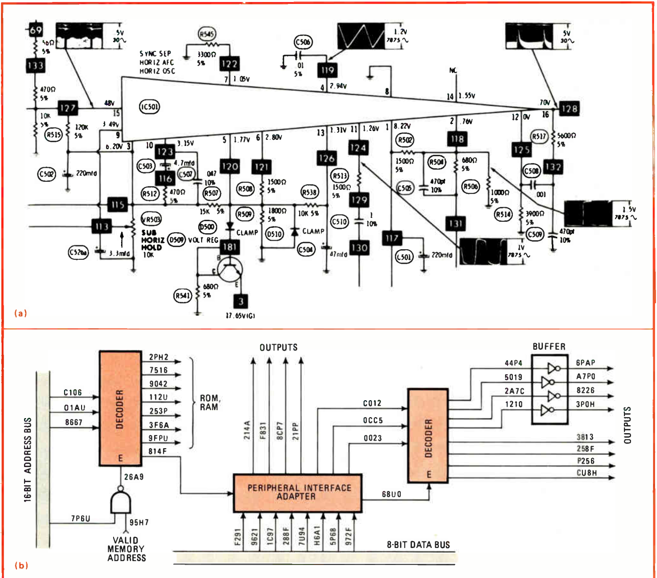
1. A new form of digital ID. Diagrams of analog circuits, as for a television set (a), have voltage levels and waveforms noted on them to aid service technicians (circuit is taken from a Howard W. Sams Photofacts service manual). But in digital circuits, all waveforms look alike, and the schematic shown here (b) is annotated instead with hexadecimal signatures that characterize the bit streams unique to each circuit node. A new test instrument derives actual signatures for the technician to compare with the correct ones on the schematic.
