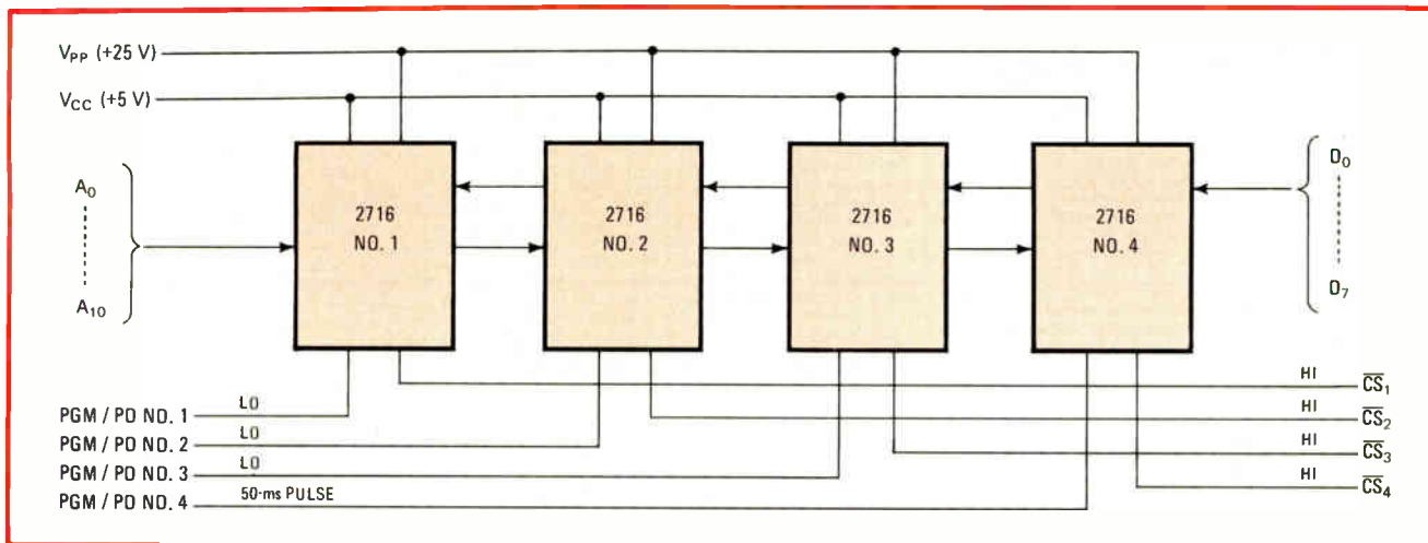
3. Picking and choosing. The 2716 erasable PROM has a program inhibit mode, to allow the designer of a multipackage system to program some of the devices and not others. Only those devices that receive a TTL-level pulse on the PGM/PD pin will be programmed.
