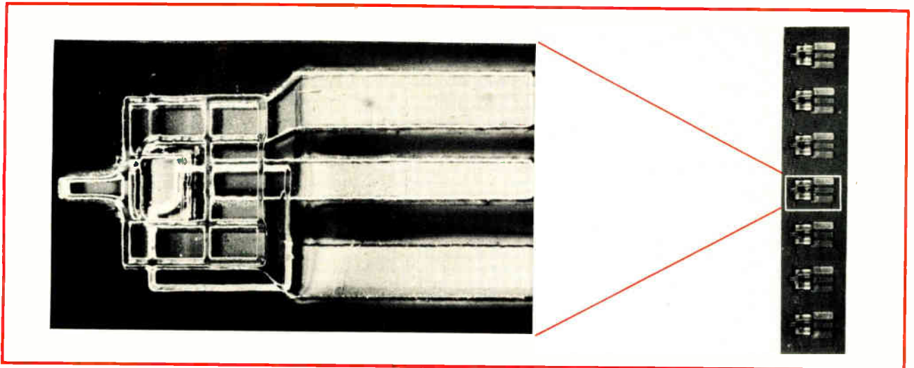
4. The sensor. A single thin-film sensor is shown in a microphotograph as viewed through the protective coating. All sensors in the linear array are deposited during a single series of vacuum depositions, allowing more precise track placement and better gap-to-gap alignment.
