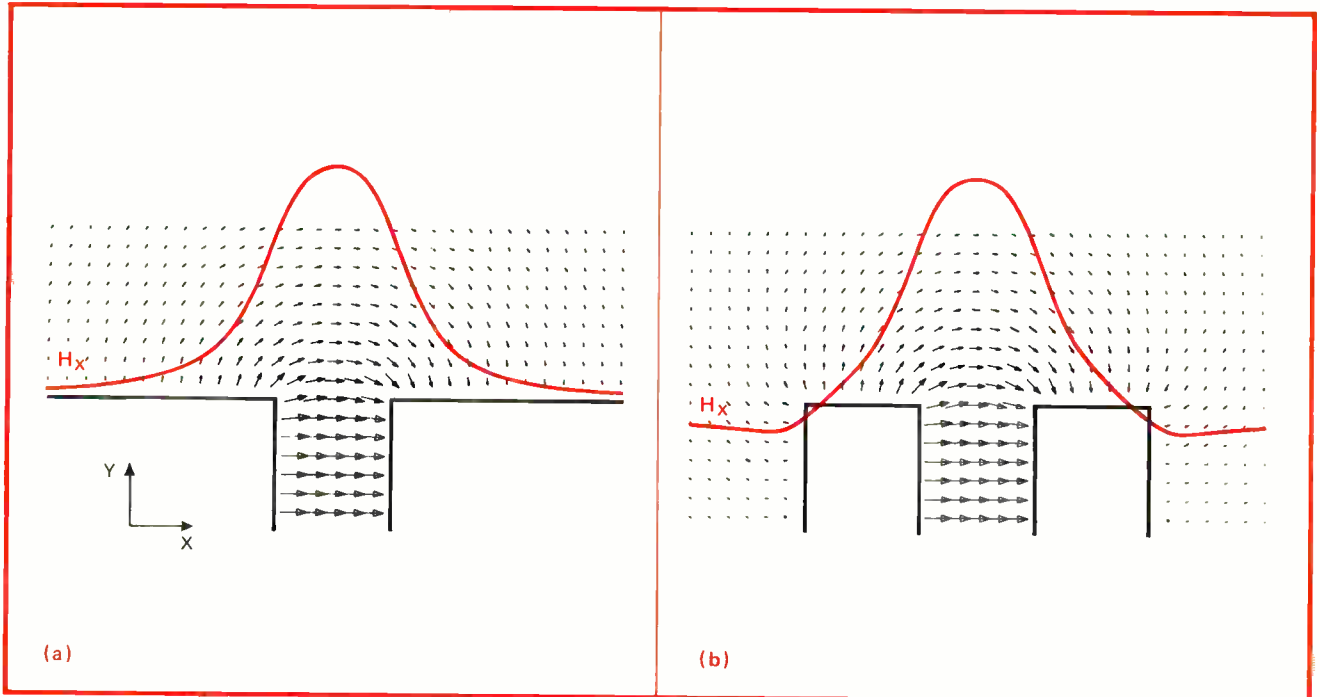
5. Fringing fields. The gap fringing fields for conventional (a) and thin-film (b) heads show the thin-film head's field has steeper sides and reaches a negative, minimum value before turning upward. Corresponding negative dips for the conventional head are far from the gap.
